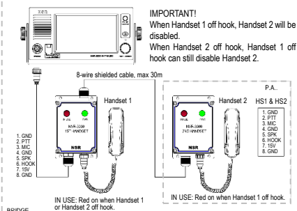
Two handsets connection (option)
