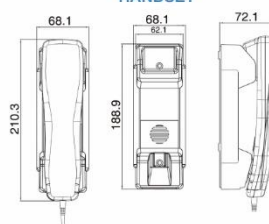
HANDSET
