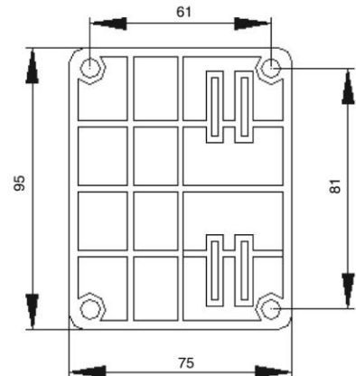
MOUNTING BRACKET
