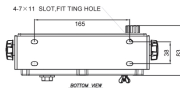
ANTENNA UNIT
